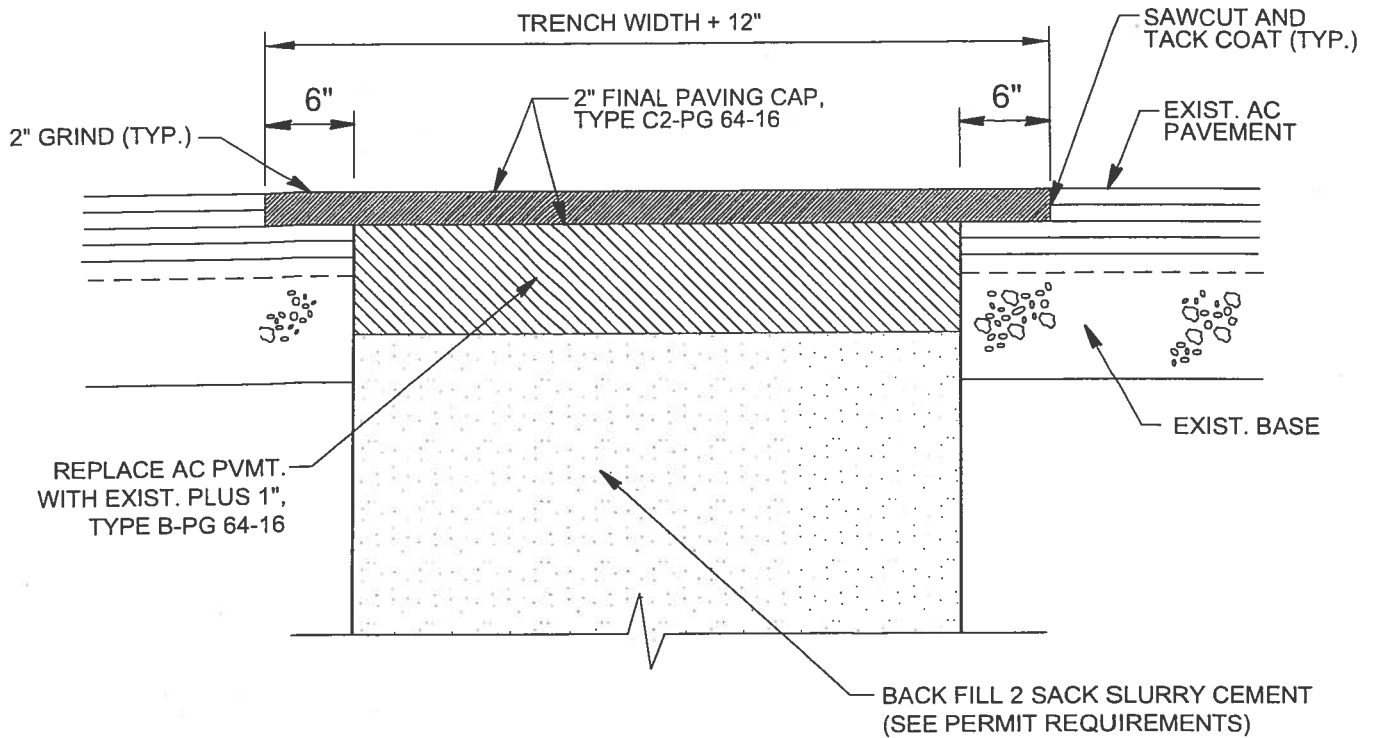
TRENCH REPAVING DETAIL
